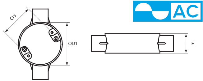
HỘP NỐI 2 ĐƯỜNG uPVC /uPVC TWO-WAY JUNCTION BOX
